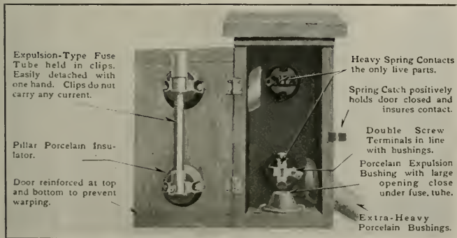
THE SAFETY FIRST FUSE BOX
